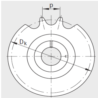
KSR...-B0
