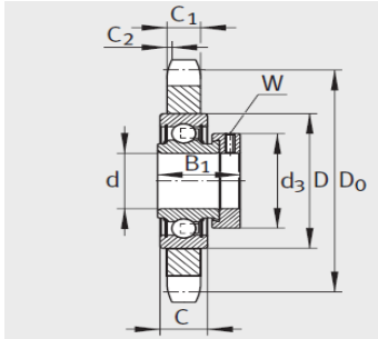
KSR...-B0
